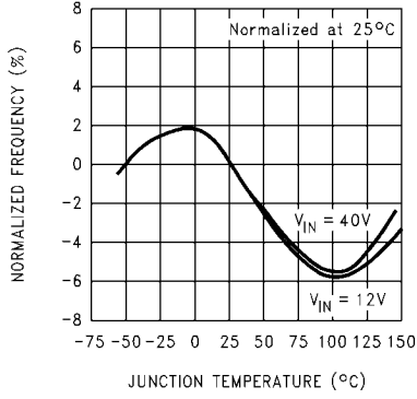
Oscillator Frequency
